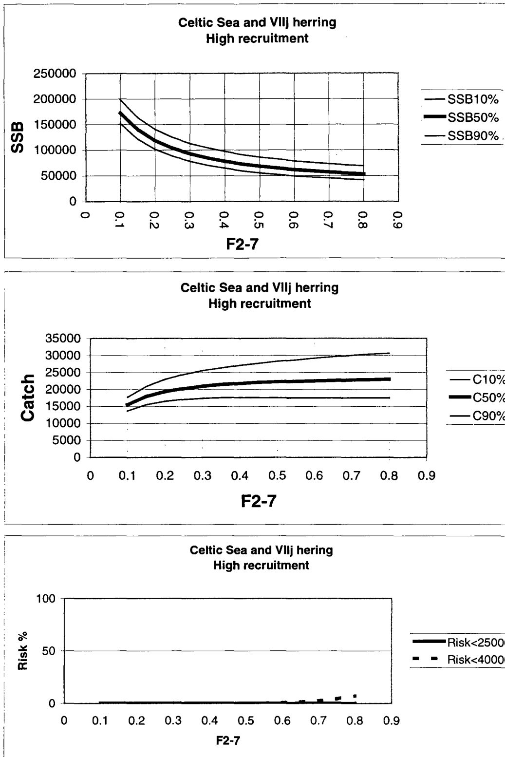
Figure 4.7.1 Long term equilibrium SSB and Catch distributions with stochastic recruitment Lower panel: Risk that SSB is below the limits indicated.
